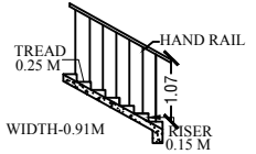
STAIRCASE DETAILS
