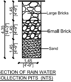
SECTION OF RAIN WATER COLLECTION PITS (NTS)
