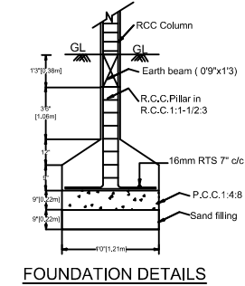
FOUNDATION DETAILS
