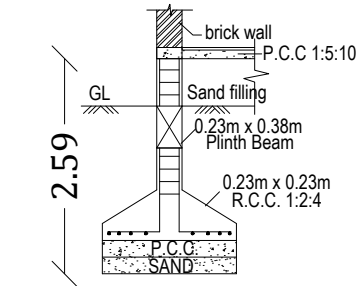
FOUNDATION DETAILS
