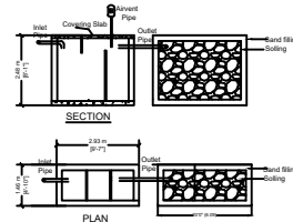
Details of solar water heating system
