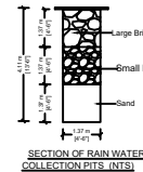
SECTION OF RAIN WATER COLLECTION PITS (NTS)
