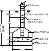
FOUNDATION DETAILS
