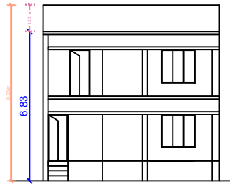
FRONT ELEVATION
