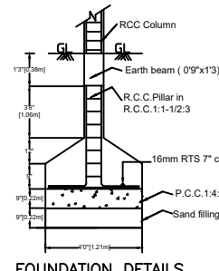
FOUNDATION DETAILS
