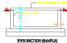
RWH_CAPACITY_L = 2000LTRS
