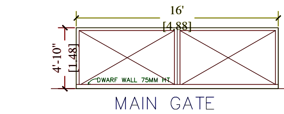
MAIN GATE
