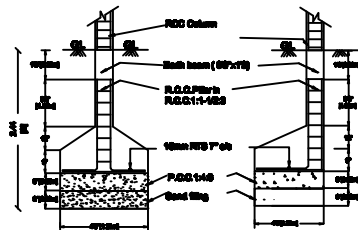
FOUNDATION DETAILS
