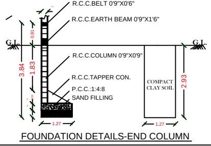
FOUNDATION DETAILS-END COLUMN
