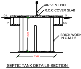
SEPTIC TANK DETAILS-SECTION
