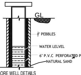
BORE WELL DETAILS
