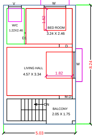
FIRST FLOOR PLAN (PROPOSED)
