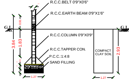
FOUNDATION DETAILS-MIDDLE COLUMN
