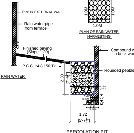
PERCOLATION PIT
