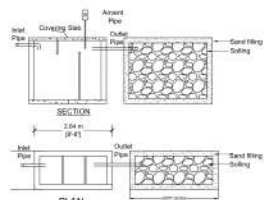
DETAILS OF SEPTIC TANK & DISPERSION TRENCH
