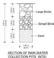
SECTION OF RAIN WATER COLLECTION PITS (N.T.S)
