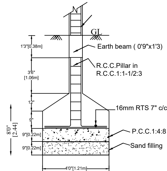
FOUNDATION DETAILS
