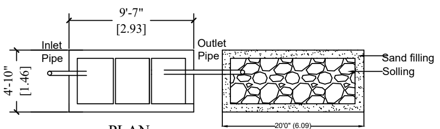
PLAN
