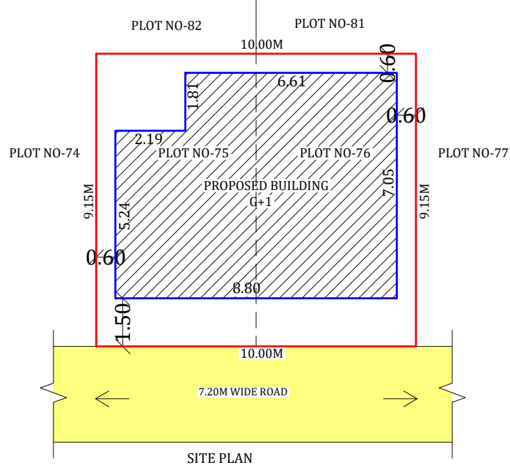
SITE PLAN
