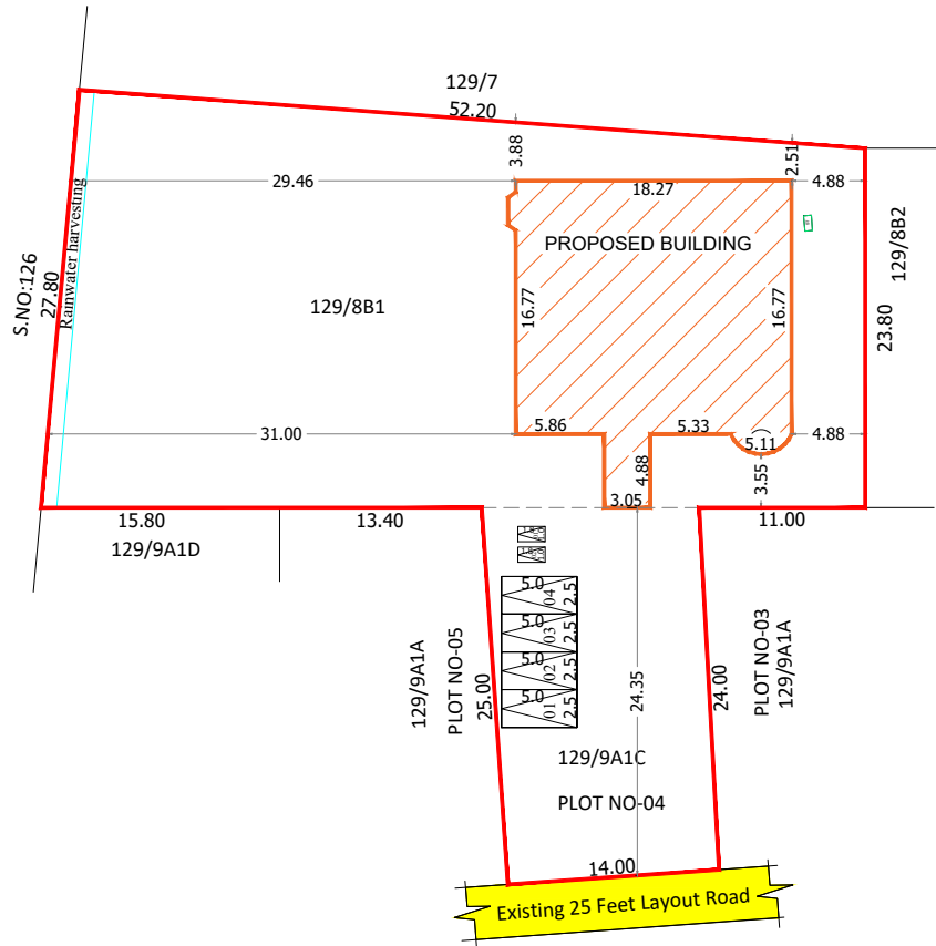
SITE PLAN
