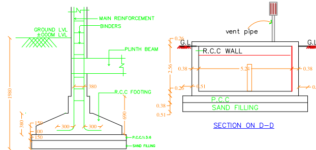
TYPICAL SECTION OF R.C.C. COLUMN FOUNDATION
