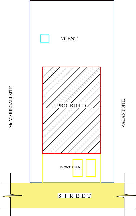
SITE PLAN
