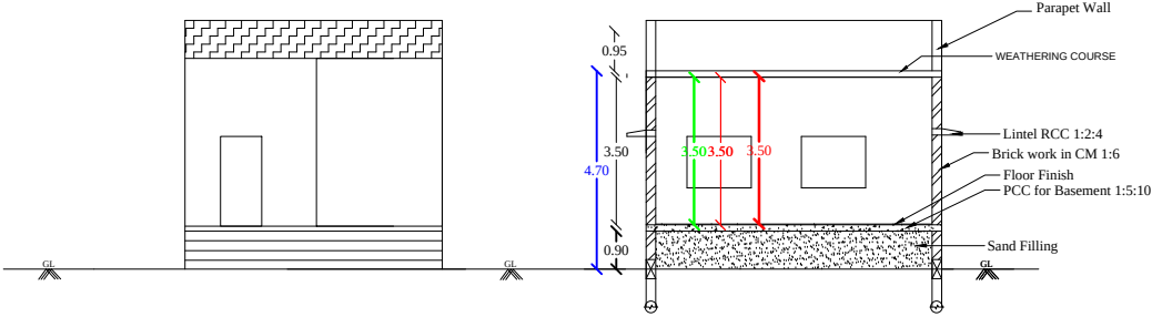
FRONT ELEVATION
