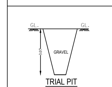
TRIAL PIT
