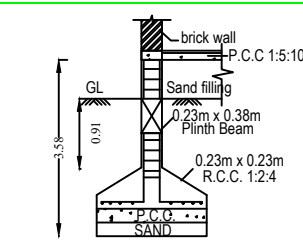
FOUNDATION DETAILS
