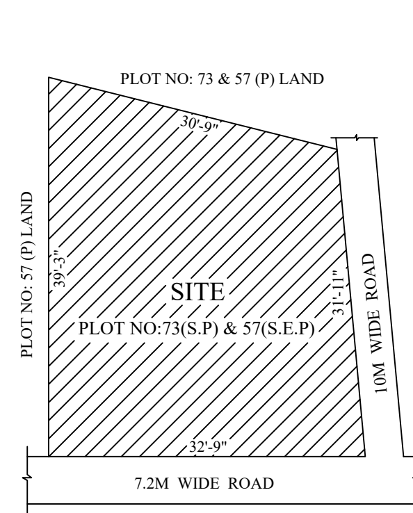
TOPO SKETCH SCALE:1" =132'
