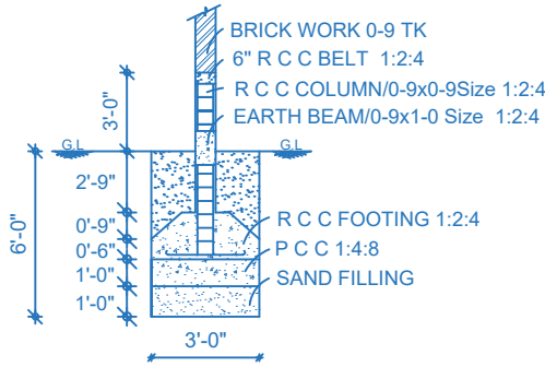
FOUNDATION
