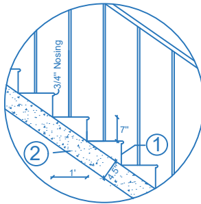
STAIRCASE SECTION
