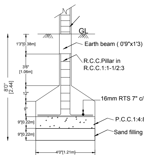
FOUNDATION DETAILS
