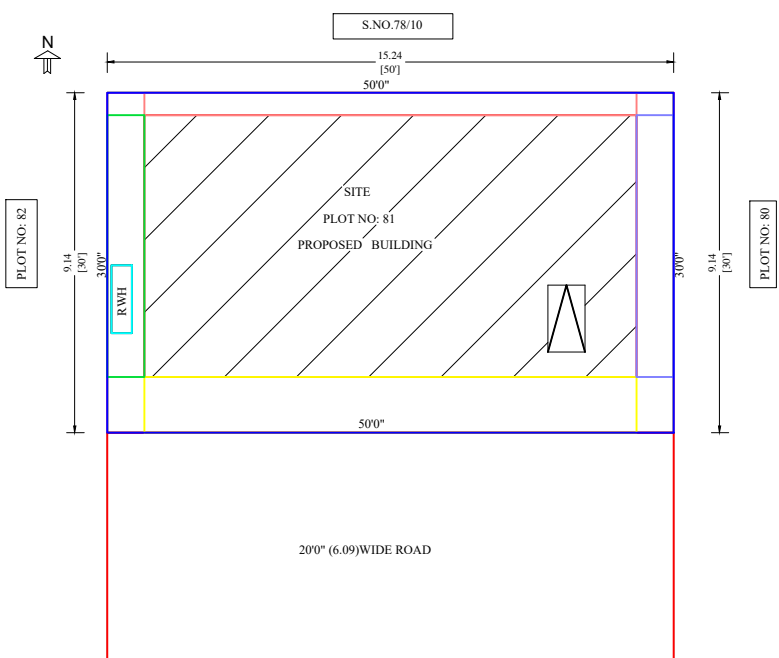
SITE PLAN
