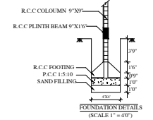
FOUNDATION DETAILS (SCALE: 1"=4'0")
