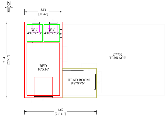
PRO.FIRST FLOOR PLAN
