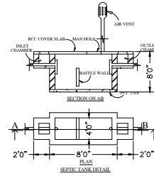
SEPTIC TANK DETAIL
