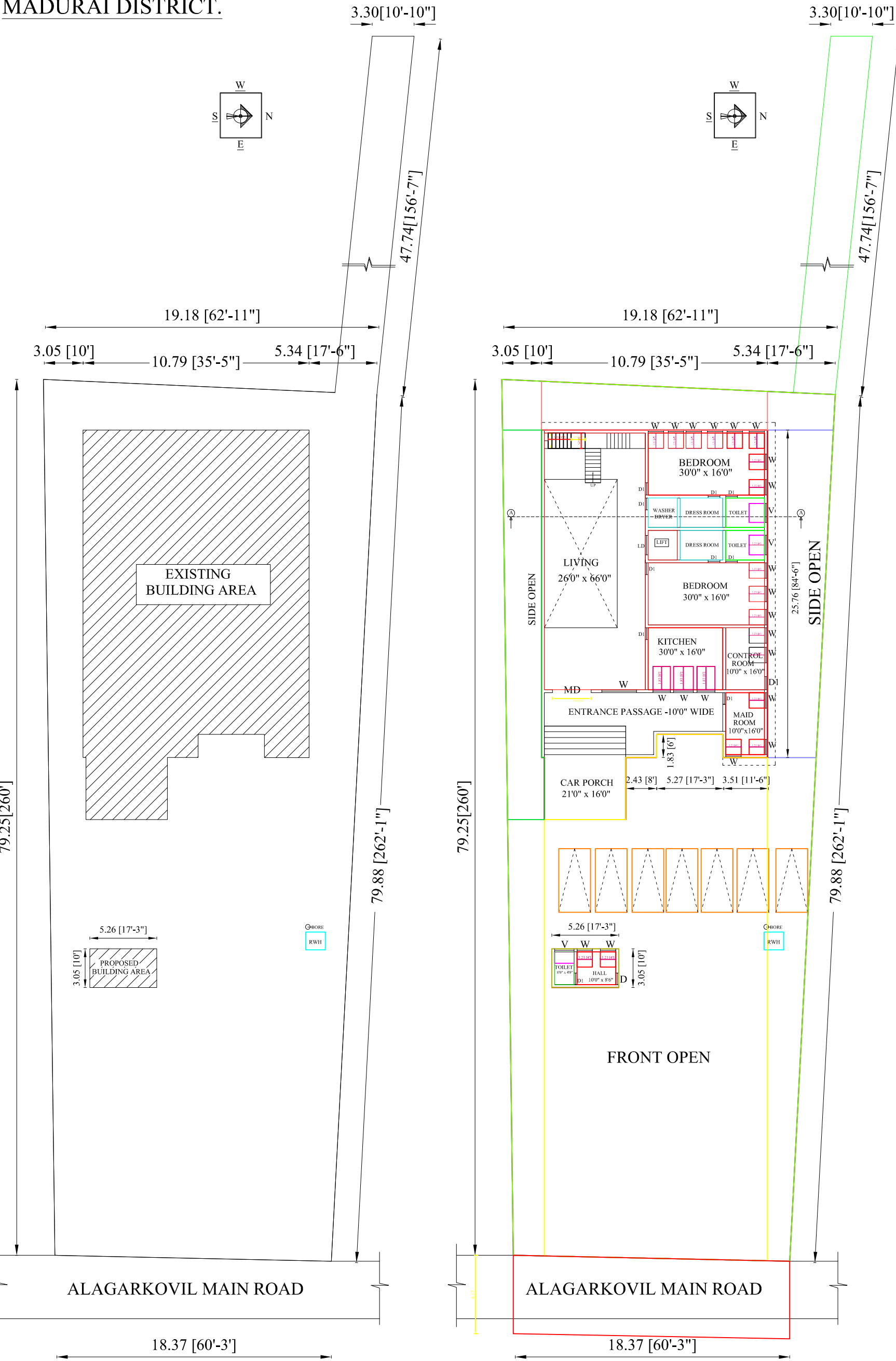
SITE PLAN
