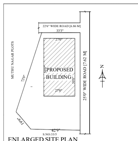
ENLARGED SITE PLAN
