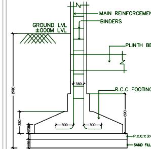
TYPICAL SECTION OF R.C.C. COLUMN FOUNDATION
