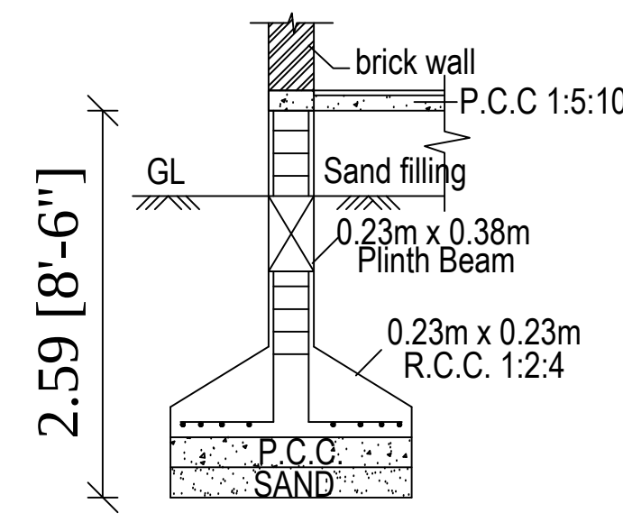
FOUNDATION DETAILS
