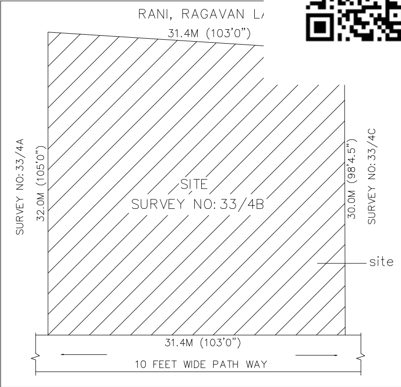
SITE PLAN
