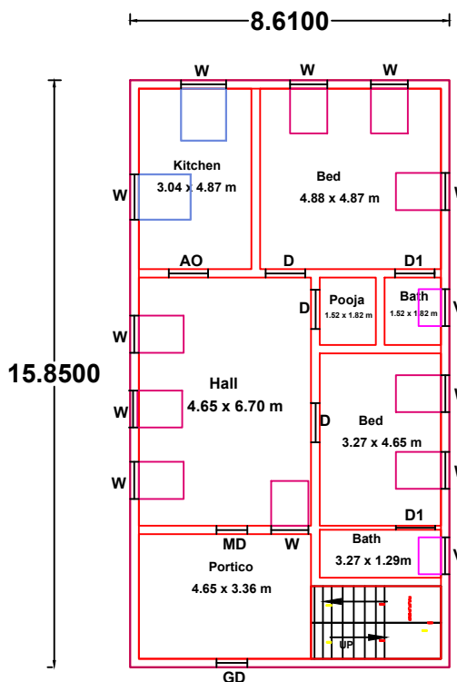
GROUND FLOOR (North Facing)
