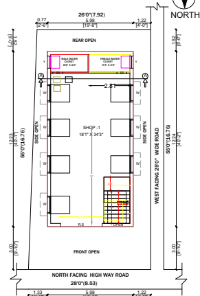
EXISTING GROUND FLOOR PLAN
