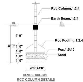
CENTRE COLUMN RCC COLUMN DETAILS
