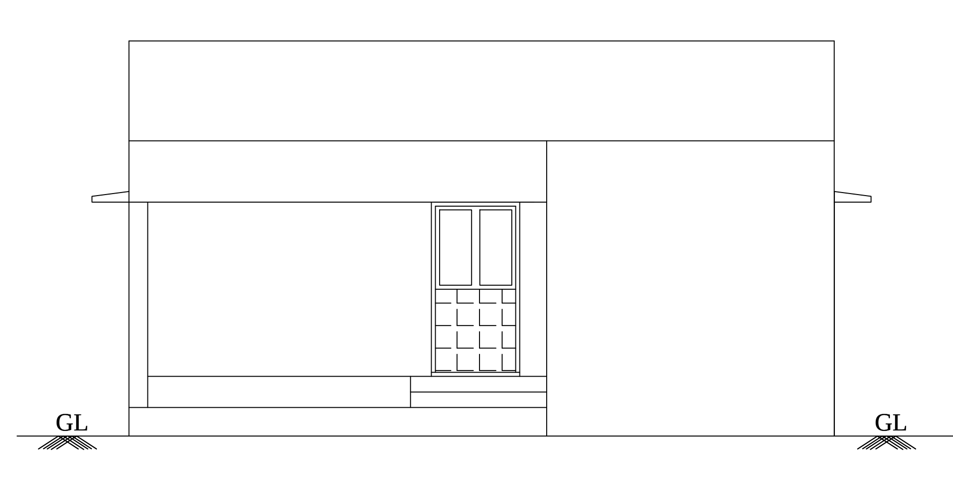
ELEVATION ON NORTH FACING
