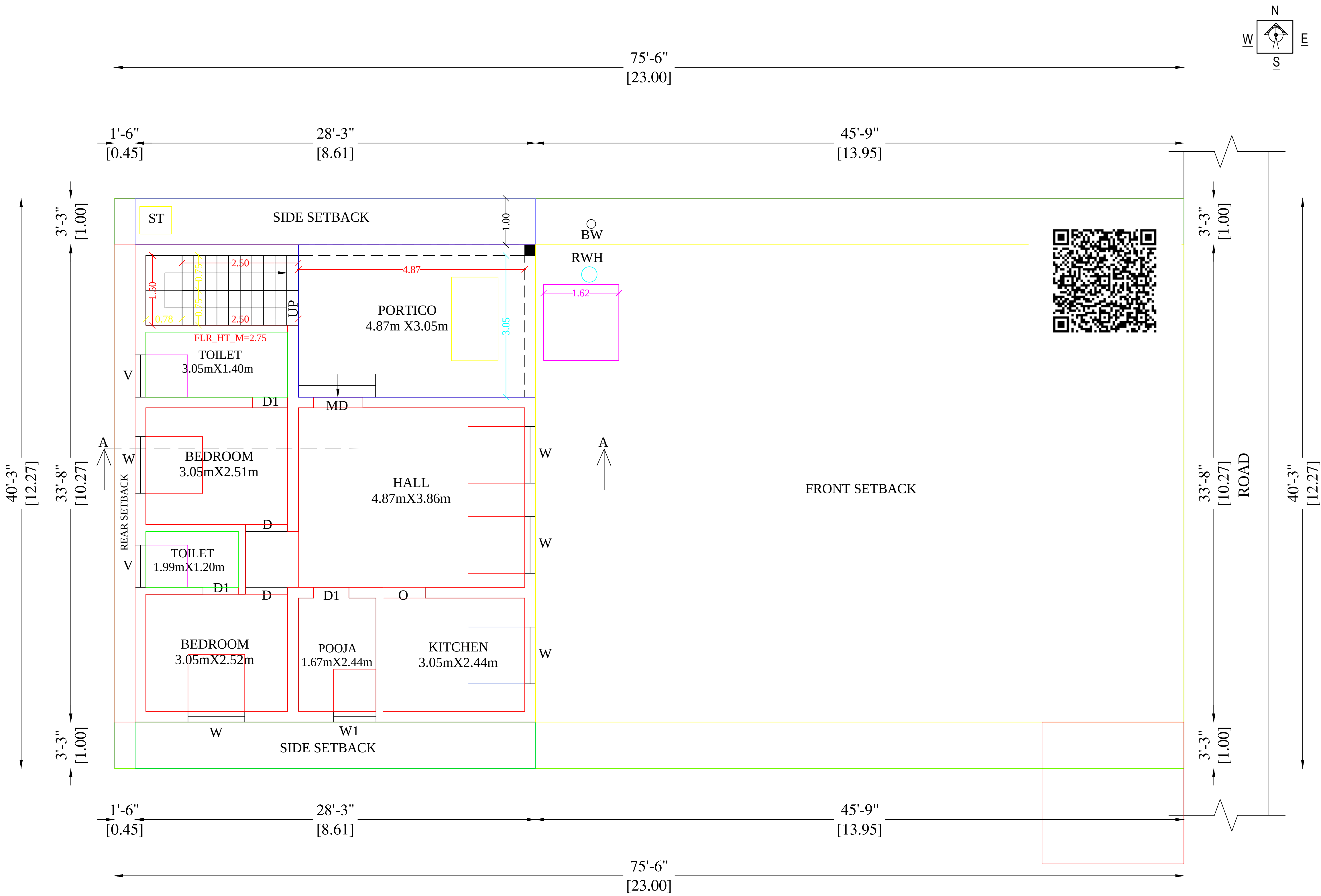
PRO. GROUND FLOOR PLAN
