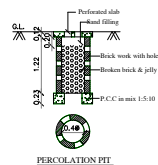
PERCOLATION PTH
