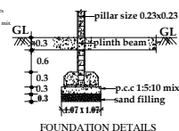
FOUNDATION DETAILS
