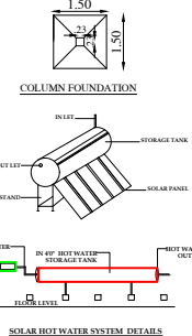
SOLAR HOT WATER SYSTEM DETAILS
