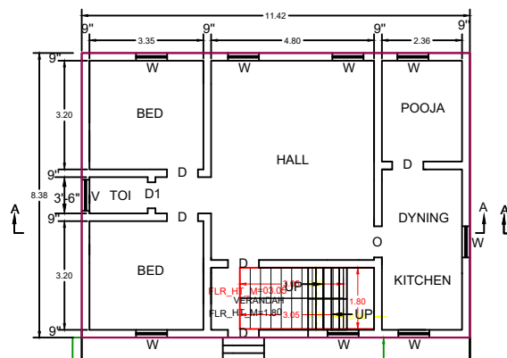
EXISTING & PROPOSED G.F. PLAN
