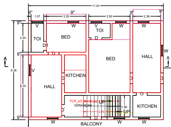
PROPOSED F.F. PLAN
