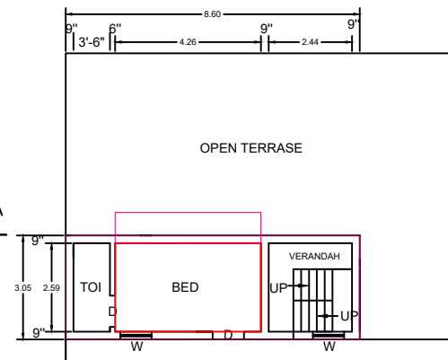
PROPOSED S.F. PLAN
