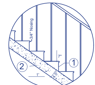
STAIRCASE SECTION Not For Scale
