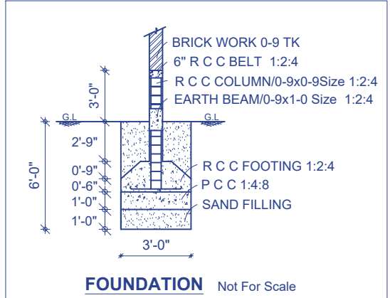
FOUNDATION Not For Scale
