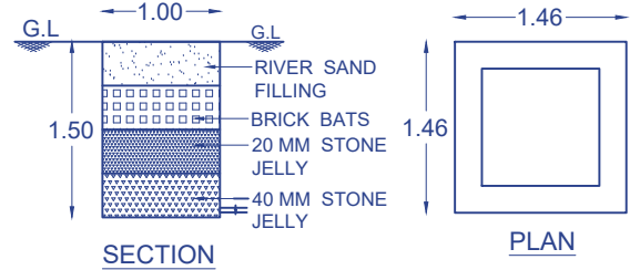
RAIN WATER HARVESTION Not For Scale
