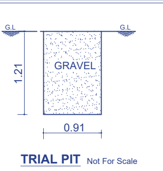
TRIAL PIT Not For Scale
