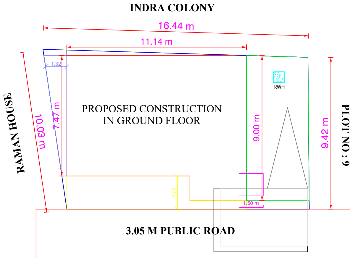
SITE PLAN
