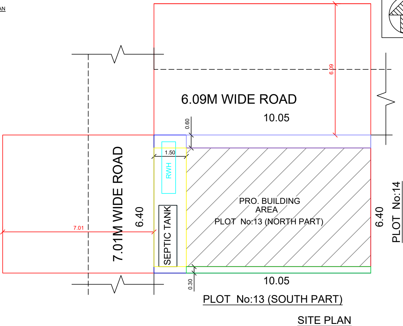
SITE PLAN
