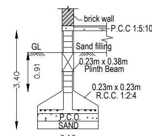
FOUNDATION DETAILS
