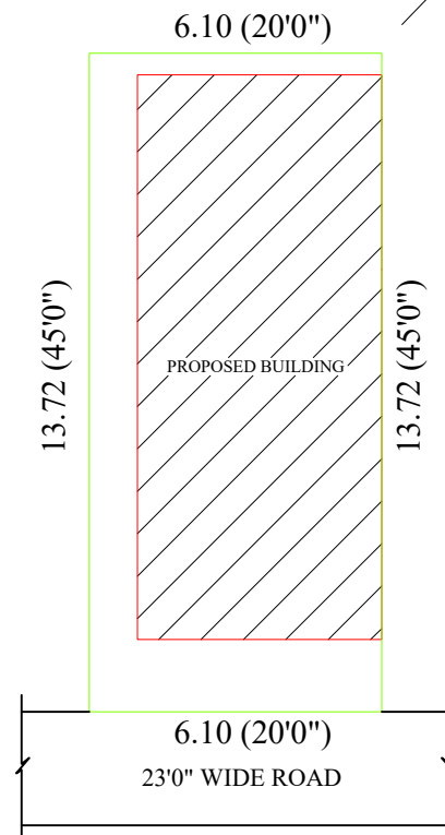
SITE PLAN
