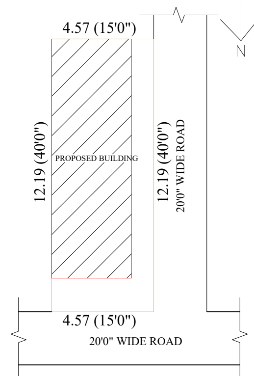
SITE PLAN
