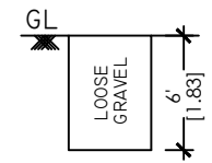
TRIAL PIT.
