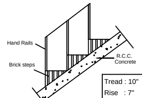
STAIRCASE DETAILS
