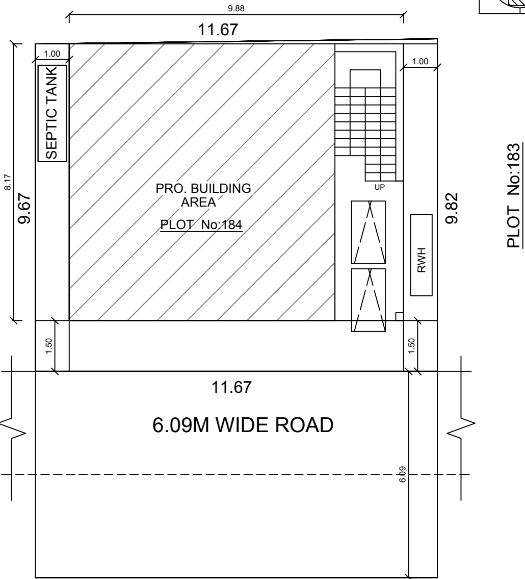
SITE PLAN
