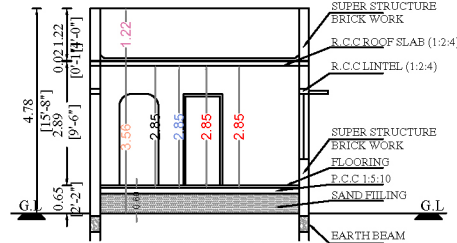
SECTION X - X
