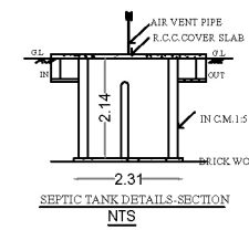
SEPTIC TANK DETAILS-SECTION NTS
