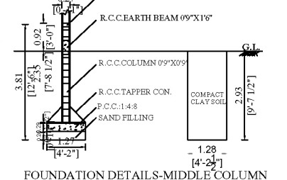
FOUNDATION DETAILS-MIDDLE COLUMN NTS
