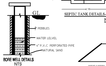
BORE WELL DETAILS NTS
