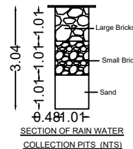
SECTION OF RAIN WATER COLLECTION PITS (INTS)
