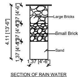
SECTION OF RAIN WATER
