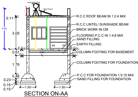
SECTION ON-AA
