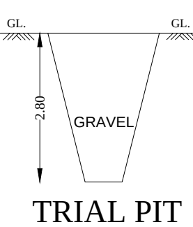
TRIAL PIT
