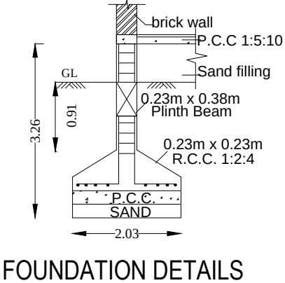
FOUNDATION DETAILS
