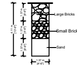
SECTION OF RAIN WATER COLLECTION PITS. (NTS)
