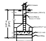
FOUNDATION DETAILS
