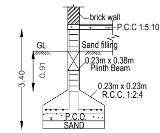
FOUNDATION DETAILS
