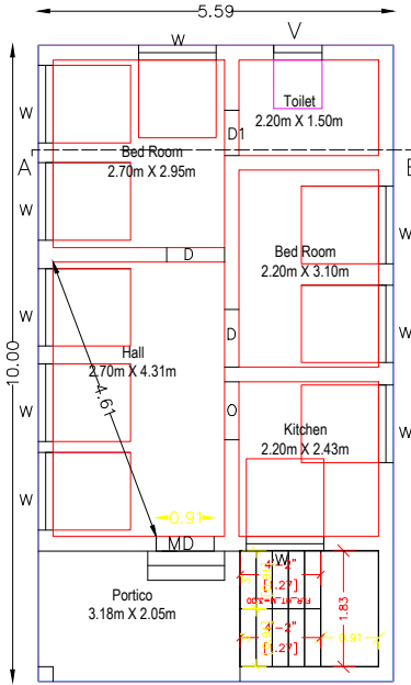
PROPOSED GROUND FLOOR
