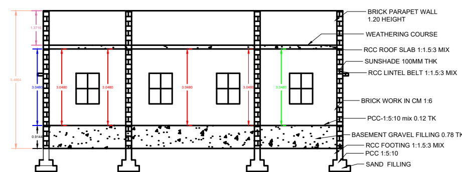
SECTION
