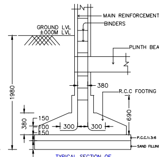
TYPICAL SECTION OF R.C.C COLUMN FOUNDATION
