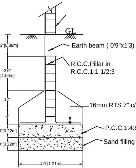
FOUNDATION DETAILS
