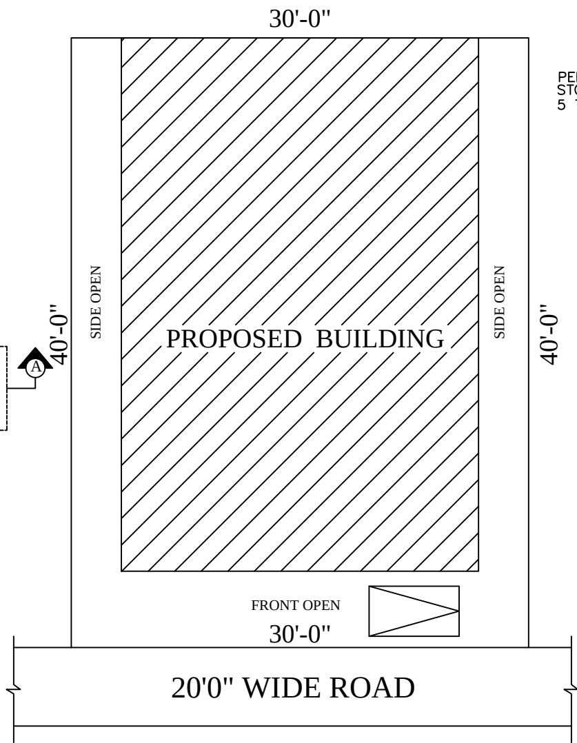
SITE PLAN
