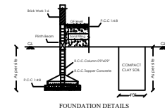
FOUNDATION DETAILS
